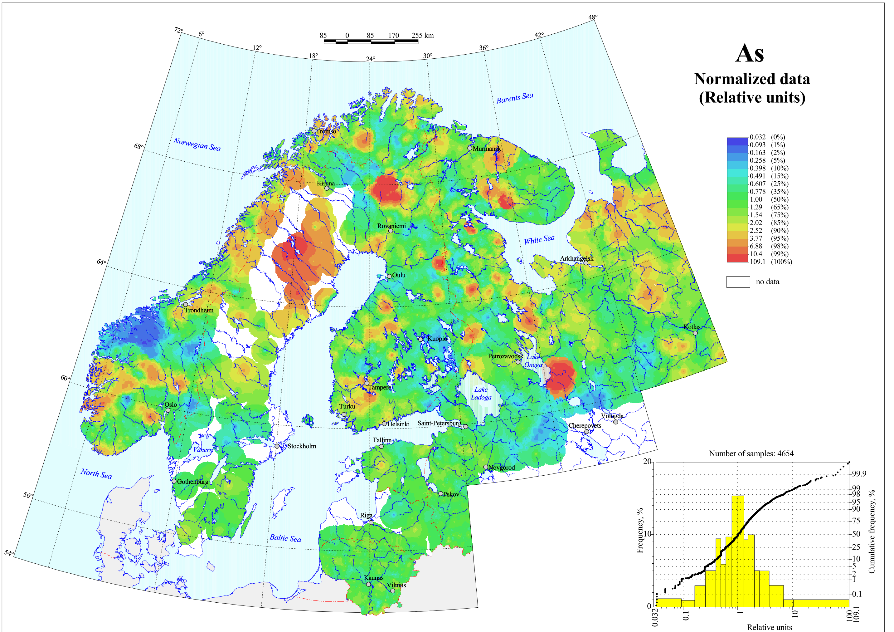
Arsenic in Stream Sediment
